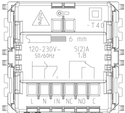
Backside view
