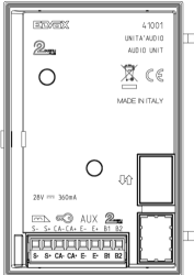
Backside view
