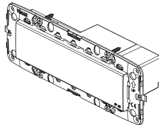
3D View
