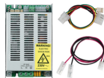
03805 - By-alarm Plus power unit 230V13Vdc3,2A
