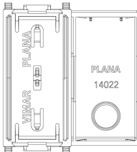
Backside view
