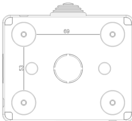
Backside view
