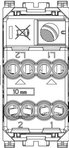
Backside view
