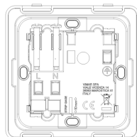
Backside view
