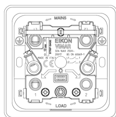
Backside view
