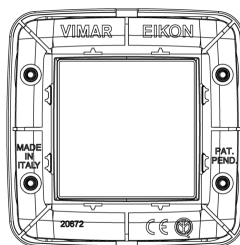
Backside view
