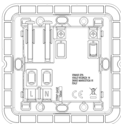
Backside view
