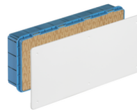
V70008 - Flush junction box 391x154x70mm
