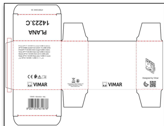
14223.C – Packaging
