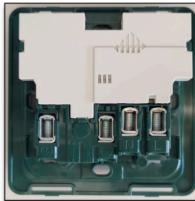
14223.C – Rear
