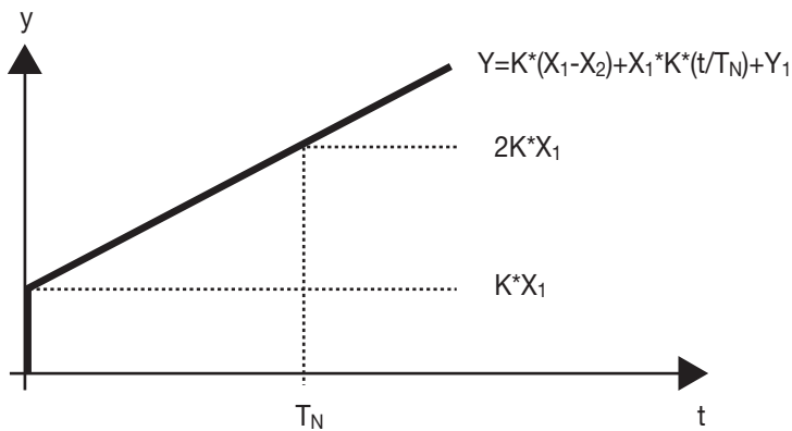
Fig. 5.7.2 (3) control value of PI control mode
