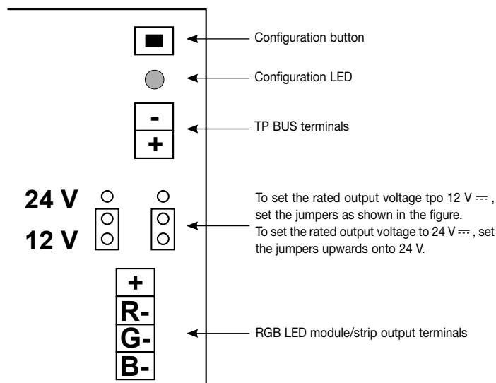
Fig. 2. Position of the jumpers to select the output voltage of 12 V \sim .
