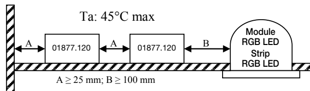
Fig. 3. Minimum distance between the power supply 01877.120 and the lamps and/or external walls.
