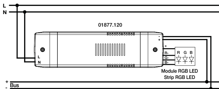
Fig. 1. Wiring diagram for power supply 01877.120.
