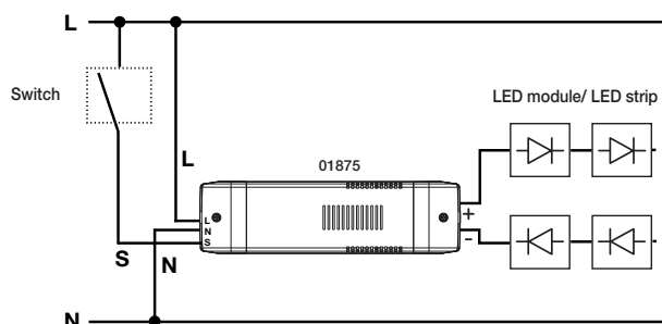
Fig. 2. Diagram of LED 350/500/700 mA dimmerable electronic power supply + ON/OFF switch connections.
