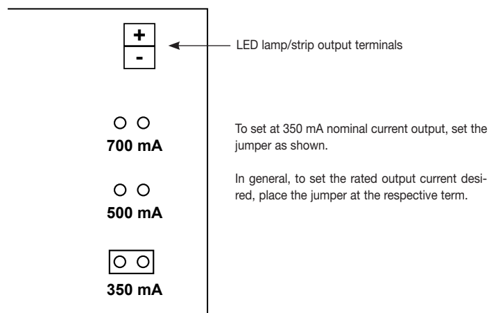
Fig. 3. Position of the jumpers for selecting the output current 350 mA
