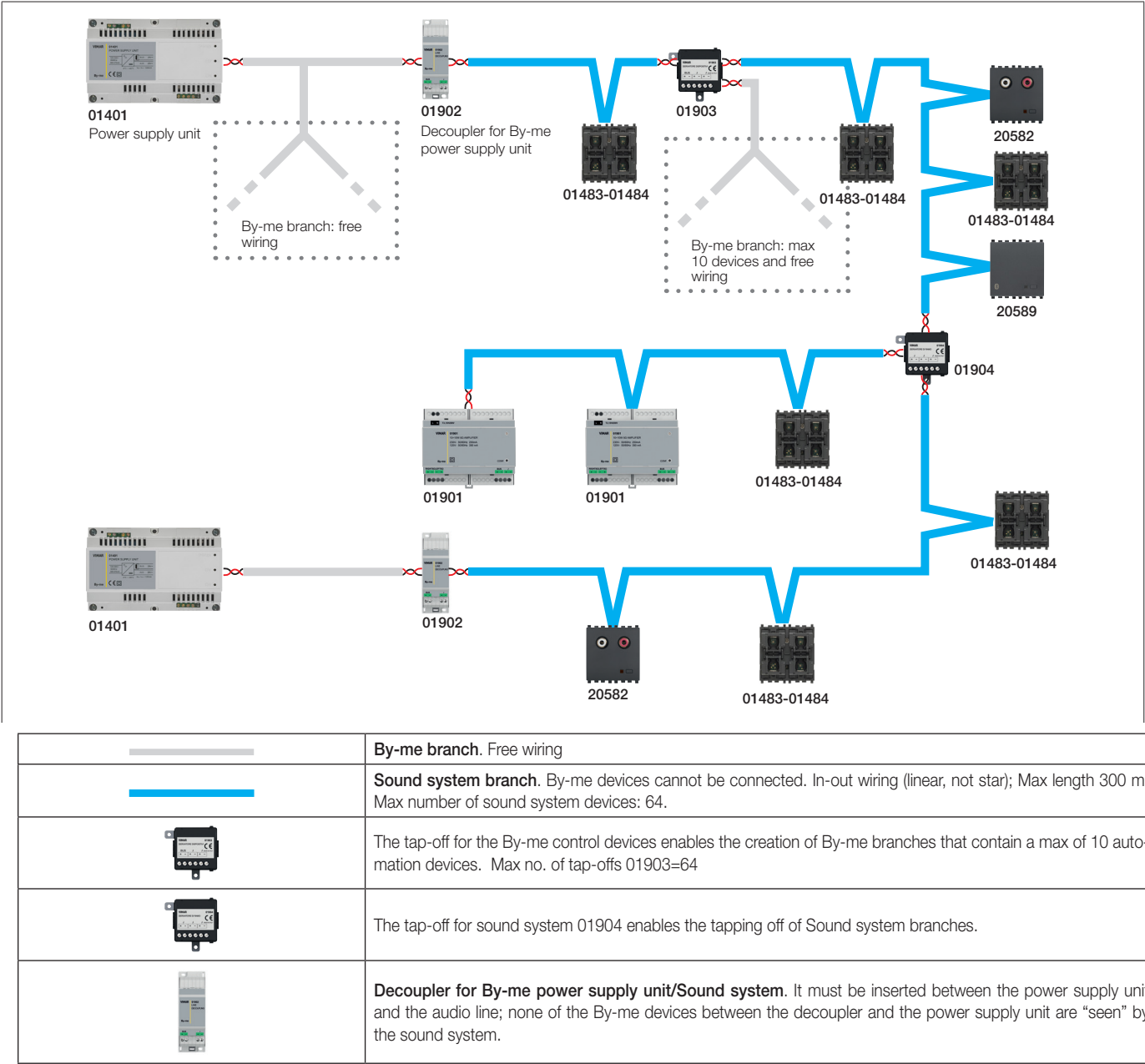
Example 3: By-me automation and sound system on the same branch
