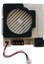
930B - Sound Sys.audio unit w/2-wire connection
