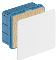
V70005 - Flush junction box 154x128x70mm
